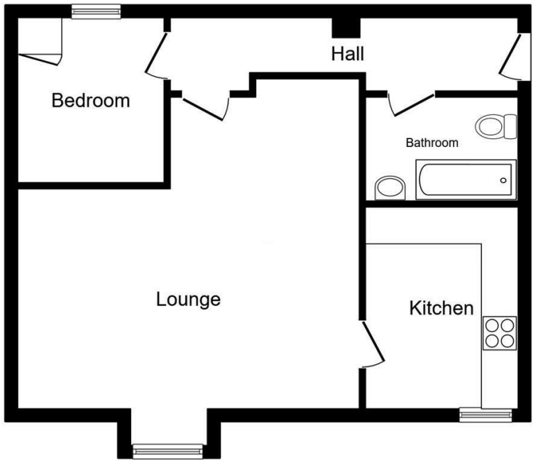
Floor Plan
